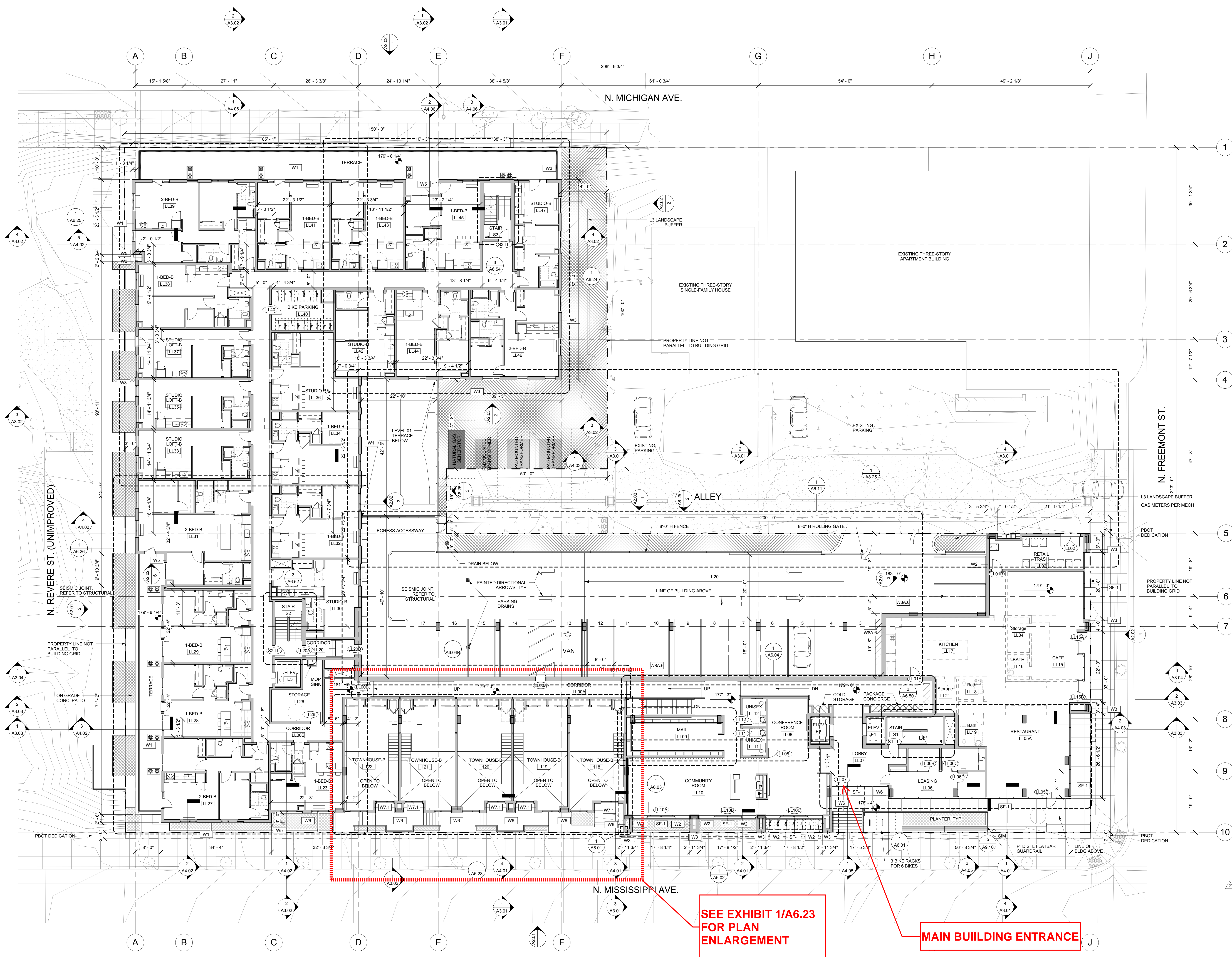
1 LOBBY LEVEL / LEVEL 1.5 FLOOR PLAN A1.01.5 3/32" = 1'-0"
