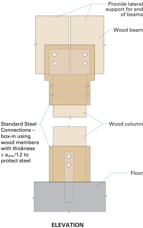
Figure 3-5 Column connections – covered
