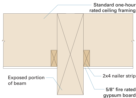
Figure 3-3 Ceiling construction
