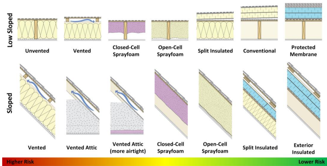
Figure 18: Relative risk of different wood-frame roof assembly options illustrating reduced risk typically associated with split insulated or exterior insulated roof assemblies. (Higher risk left (red) and lower risk (green) right) 10
