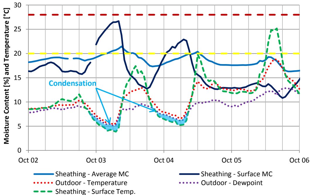
Figure 15: Chart showing fluctuations in sheathing moisture content over the course of four days in October, 2013. Note during two night the sheathing temperature drops below the ambient dew point temperature of the air creating wetting events which are also reflected in the increased moisture content during these periods. During the day time the sheathing surface temperature is often greater than the ambient outdoor temperature due to solar heat gains, and associated drying occurs.
