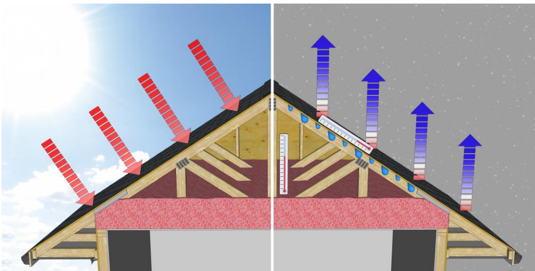
Figure 12: Graphic representation of solar heat gains on a roof during the day which would cause the roof sheathing temperature to increase (left) and of radiation to the sky at night causing the temperature of the roof sheathing to drop below the ambient air temperature and potentially cause condensation on the underside of the sheathing if it drop below the air dewpoint temperature.
