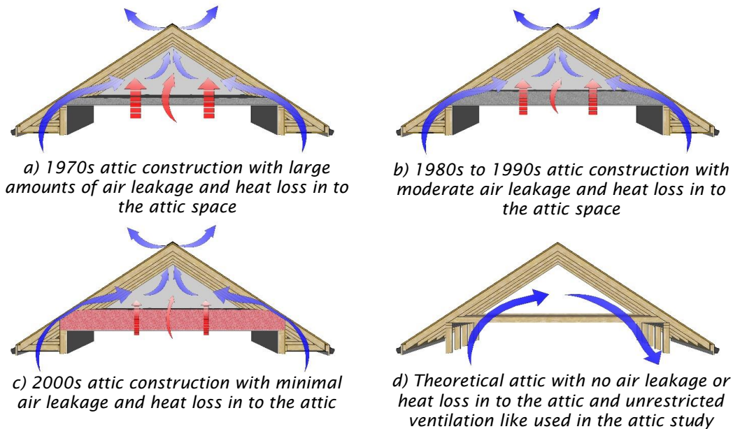
Figure 17: Schematics showing historical ventilation, insulation, and air leakage arrangements for attics (a, b, and c) and for a theoretical attic (d). Blue lines represent ventilation airflow into and out of the attics, red dashed lines and curved lines represent heat loss and air leakage respectively into the attics from the interior.
