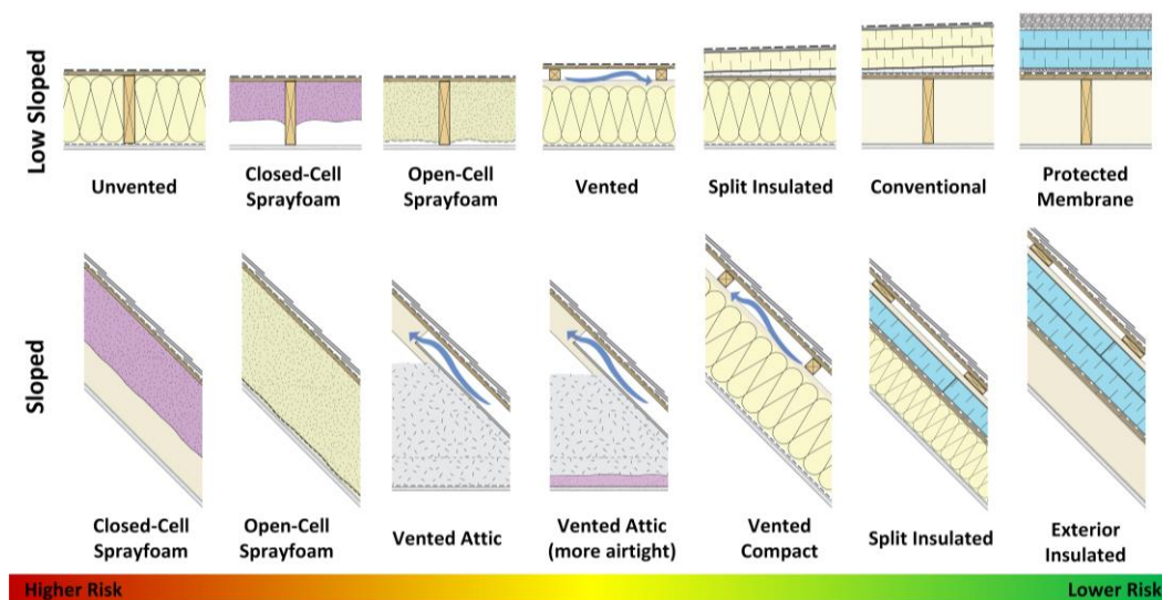
Figure 10: Relative risk of different wood-frame roof assembly options illustrating reduced risk typically associated with split insulated or exterior insulated roof assemblies. (Higher risk left (red) and lower risk (green) right) 5
