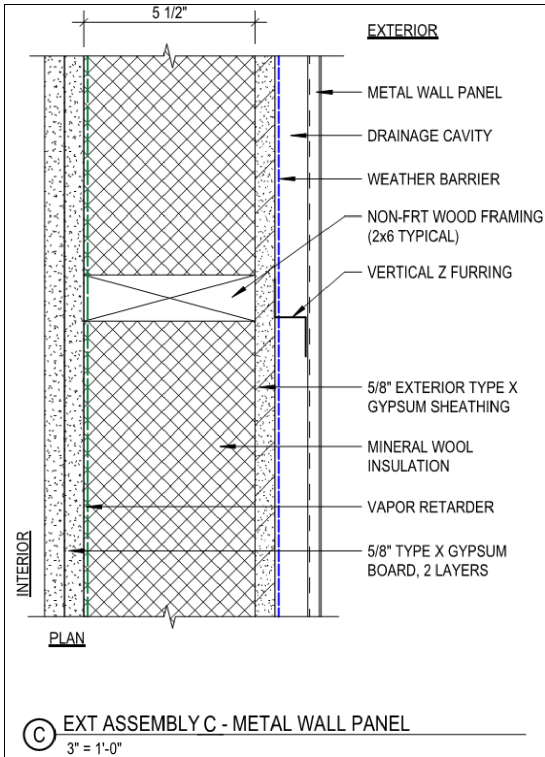
Appendix A; Figure 4: Type C-Exterior Wall
