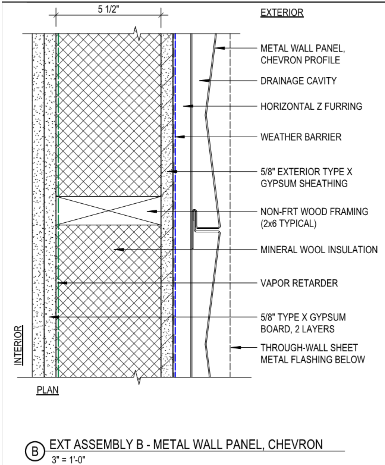
Appendix A; Figure 3: Type B-Exterior Wall
