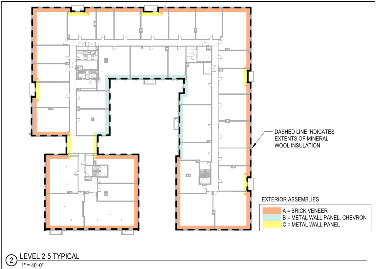
Appendix A; Figure 1: Floor Plan Showing the Location of Mineral Wool Filled Exterior Walls
