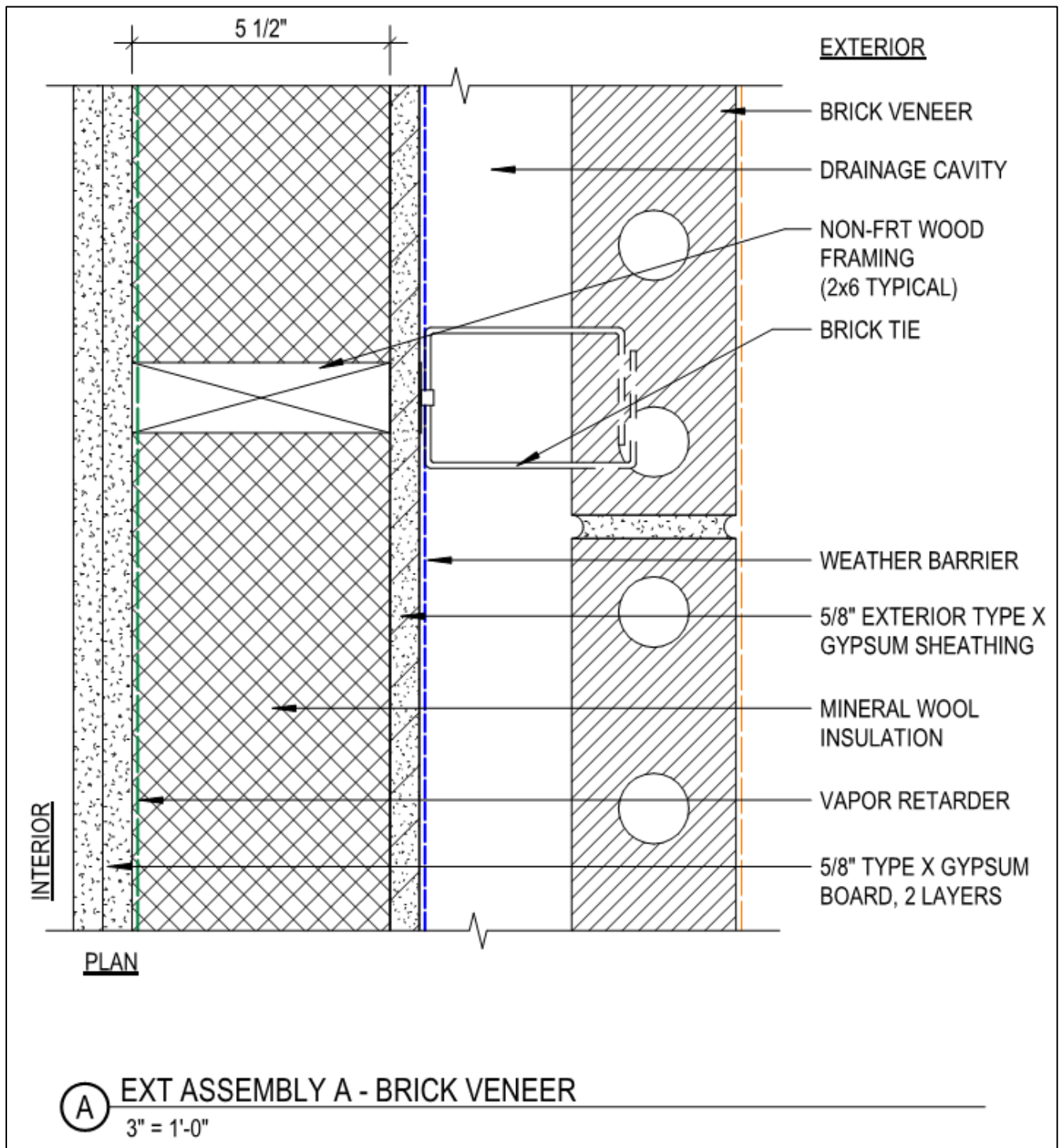
Appendix A; Figure 2: Type A-Exterior Wall
