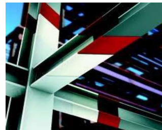
Figure 3 – Steelwork Fire Protected By SFRM Coating System (Photo Courtesy Of GCP Applied Technologies)
