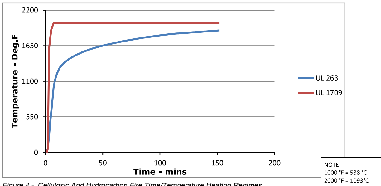
Figure 4 - Cellulosic And Hydrocarbon Fire Time/Temperature Heating Regimes
