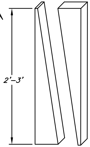
TYPICAL DEAD STOUT STAKE SAW 2X4 LUMBER ON DIAGONAL
