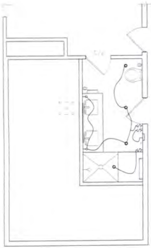
(B) ATTIC BATH ELECTRIC/RCP 1/4" = 1'-0"
