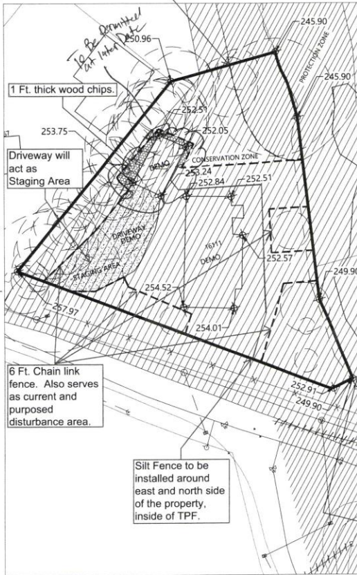
SITE PLAN
