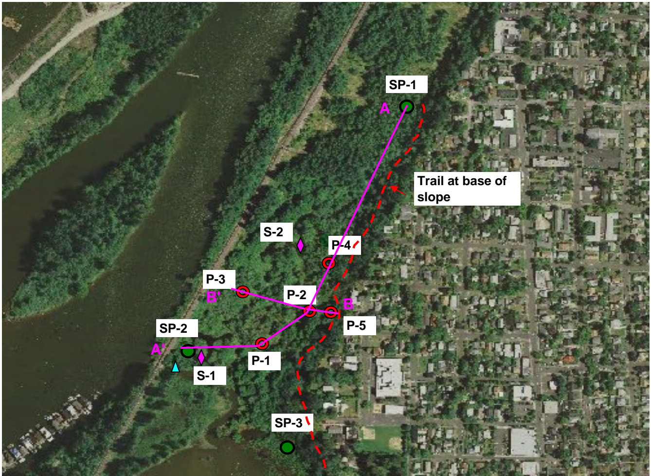
Piezometer and Staff Gauge Locations Oaks Bottom BES 8576
