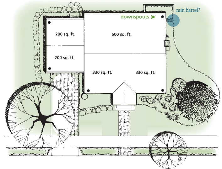
example site plan: locate existing downspouts
