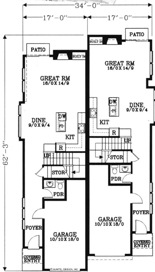
MAIN FLOOR PLAN 717 SQUARE FEET 1628 TOTAL SQUARE FEET
