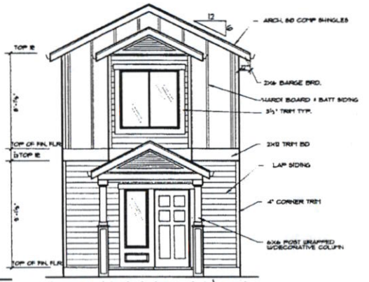
FRONT ELEVATION UNIT 1
