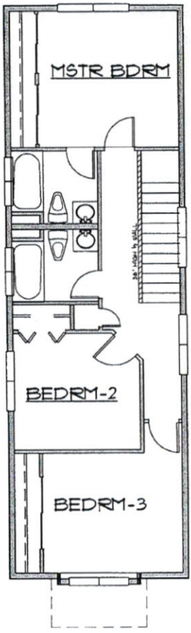
SECOND FLOOR
