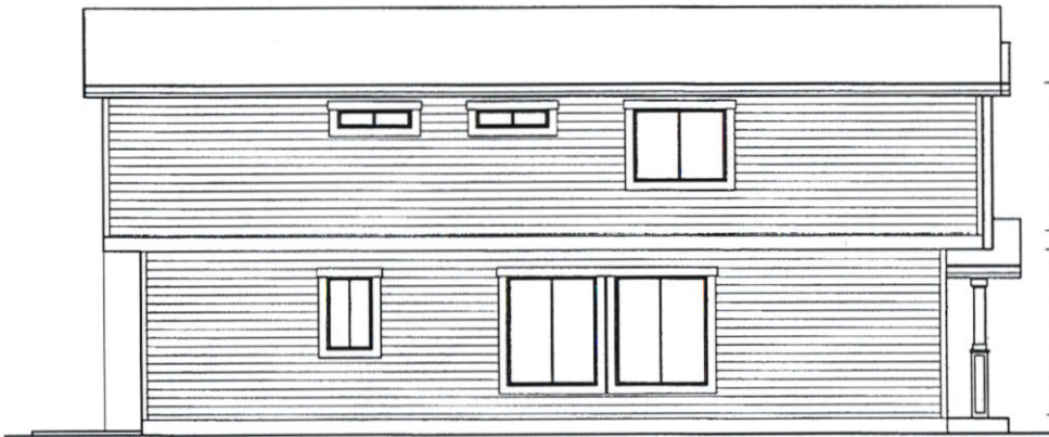
LEFT ELEVATION
