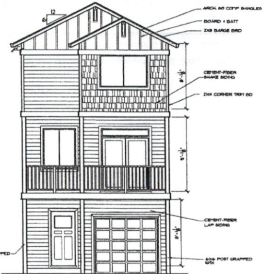
FRONT ELEVATION
