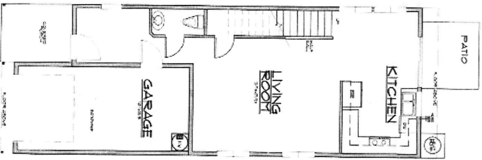
MAIN FLOOR PLAN
