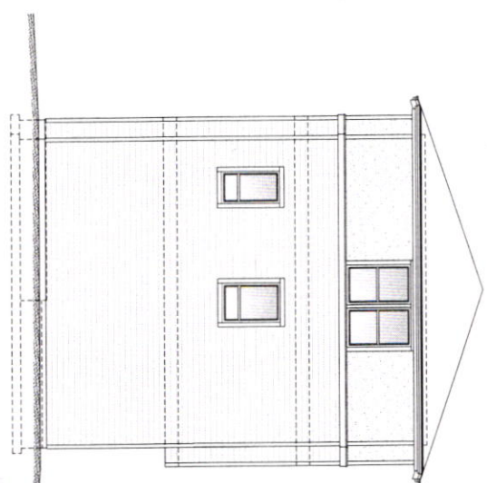
2 SOUTH BUILDING ELEVATION SCALE 1/4" = 1'-0"
