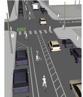
A. Left-side buffered bike lane
