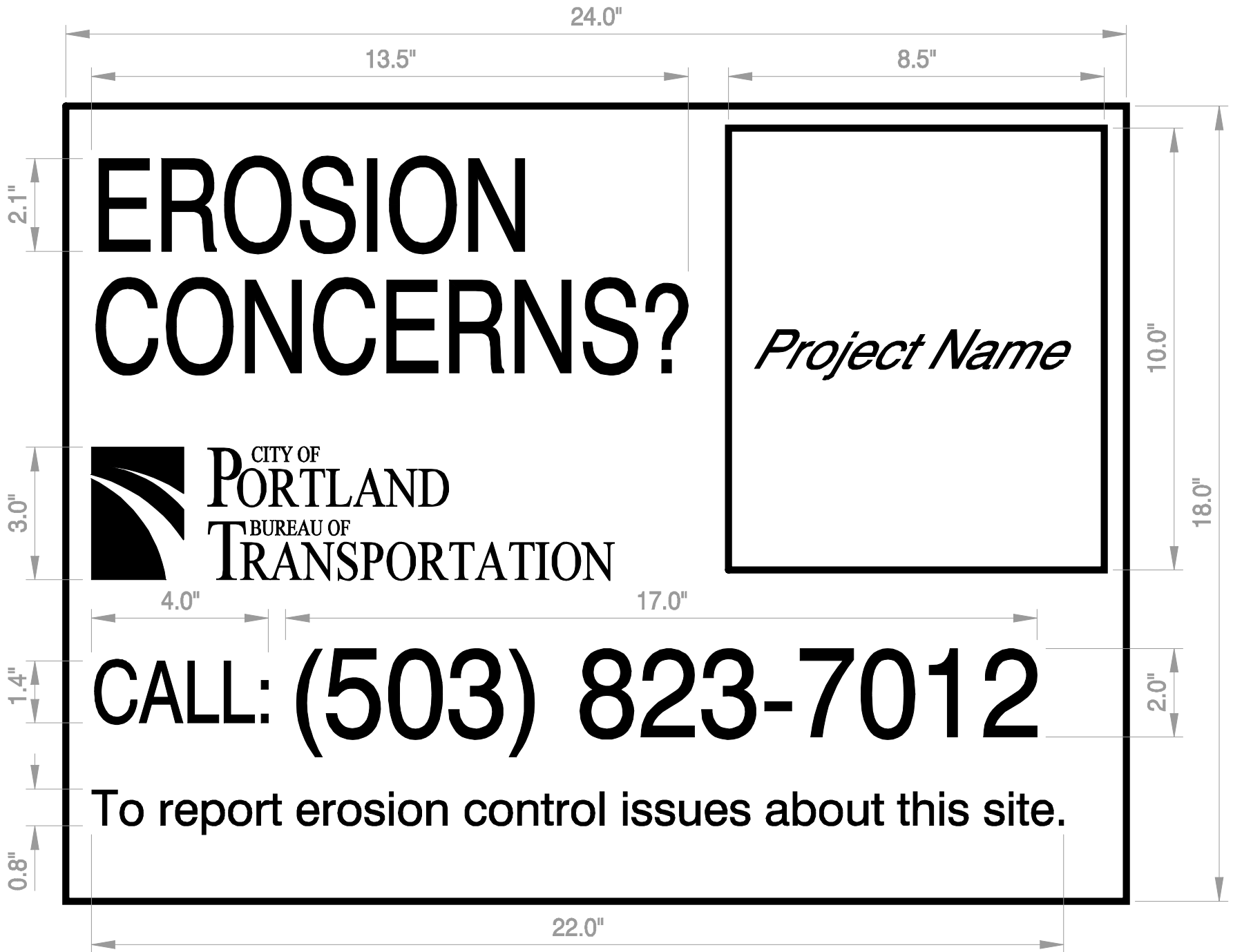
Type "O4" Sign
